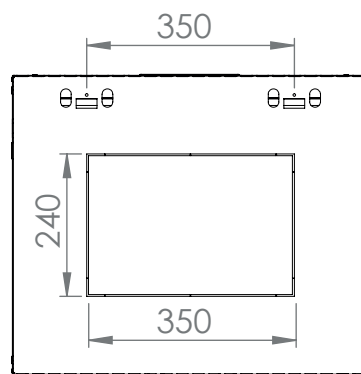
DIMENSIONS IN WIDTH AND HEIGHT
