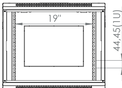
DIMENSIONS IN WIDTH AND HEIGHT
