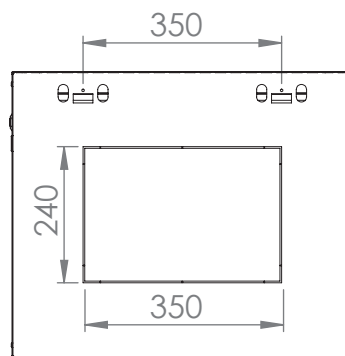
DIMENSIONS IN WIDTH AND HEIGHT
