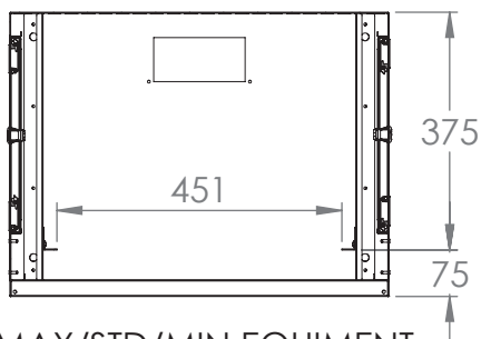
MAX/STD/MIN EQUIPMENT MOUNTING DISTANCE
